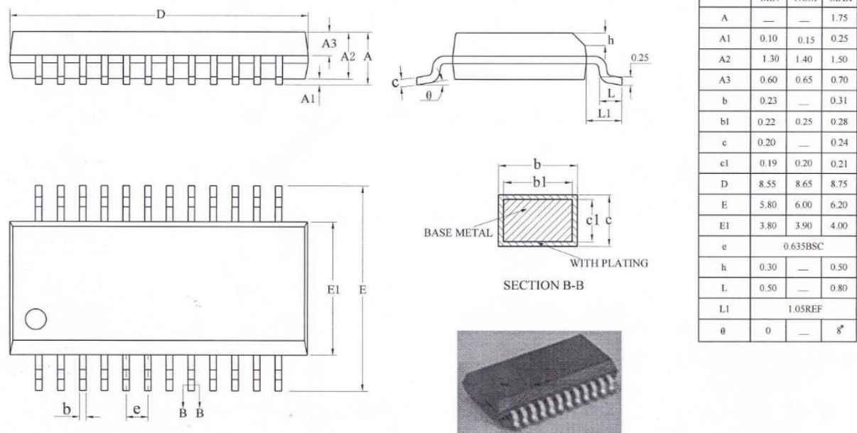
Figure 3-1. AC6925A_QSOP24 Package
